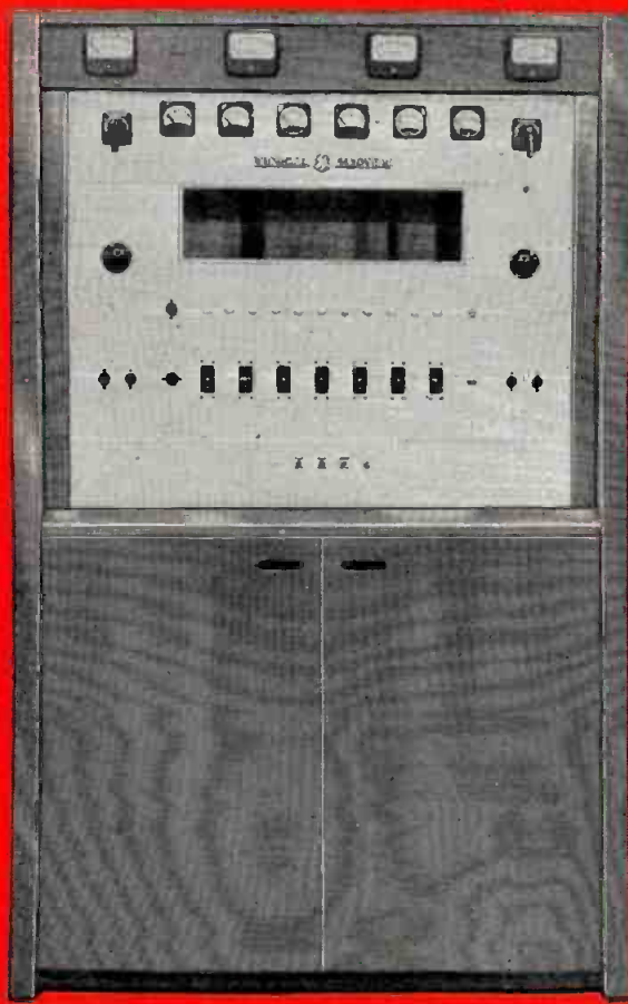
General Electric's 20 KW Amplifier Left, Visual Cubicle... Right, Aural Cubicle
